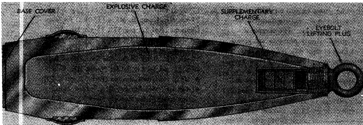
Fig 1-3 TYPICAL HE PROJECTILE W/SUPL CHARGE
